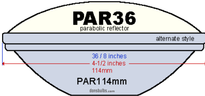
typical photo of 4509 13V 100W USA bulb type (your bulb may look slightly different)
