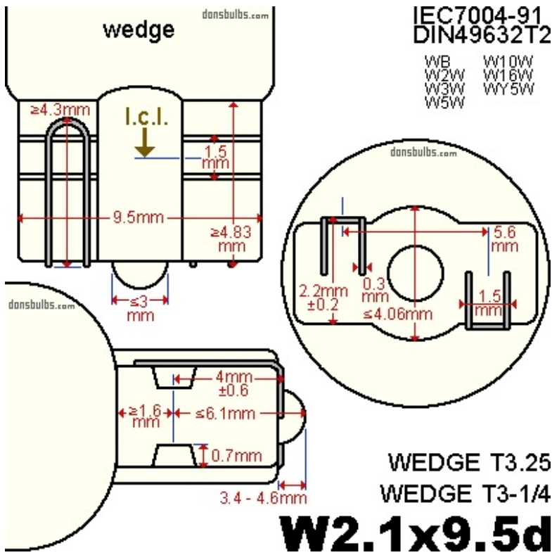
industry standards for base: W2.1x9.5d (not to scale)
